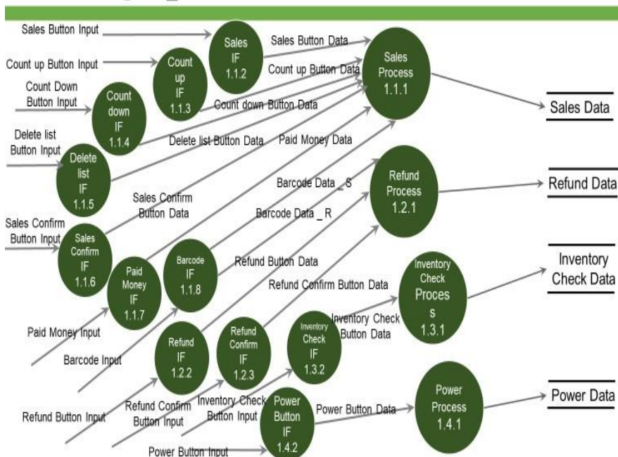
Data Flow Diagram _ Level 3
