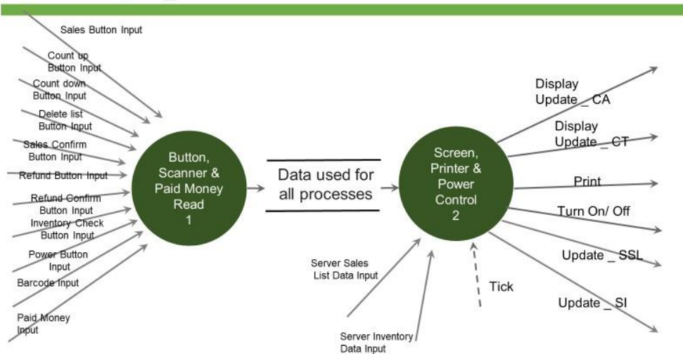
Data Flow Diagram Level 1
