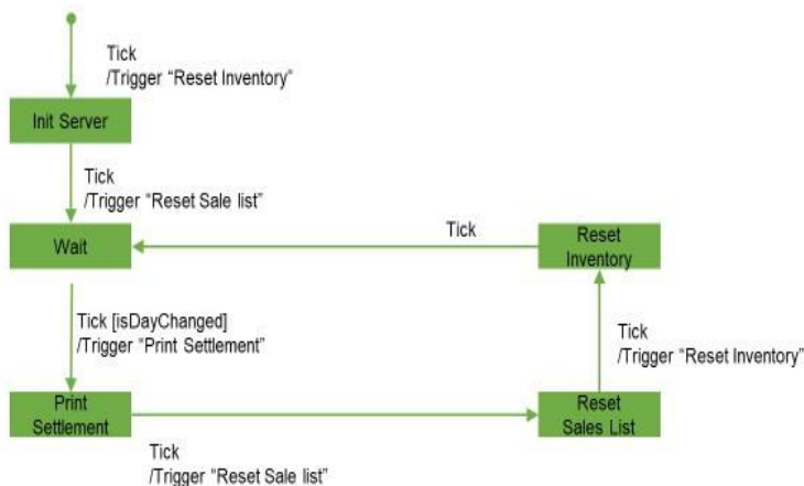
State Transition Diagram (Periodic Settlement Controller)
