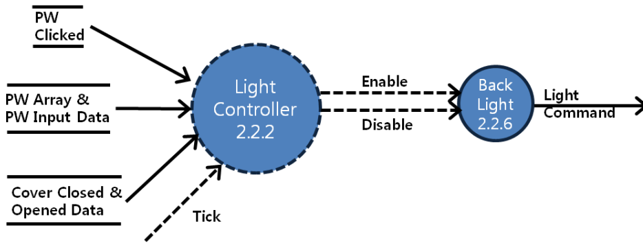
3.2.4.1.5 DFD overall for Level 3
