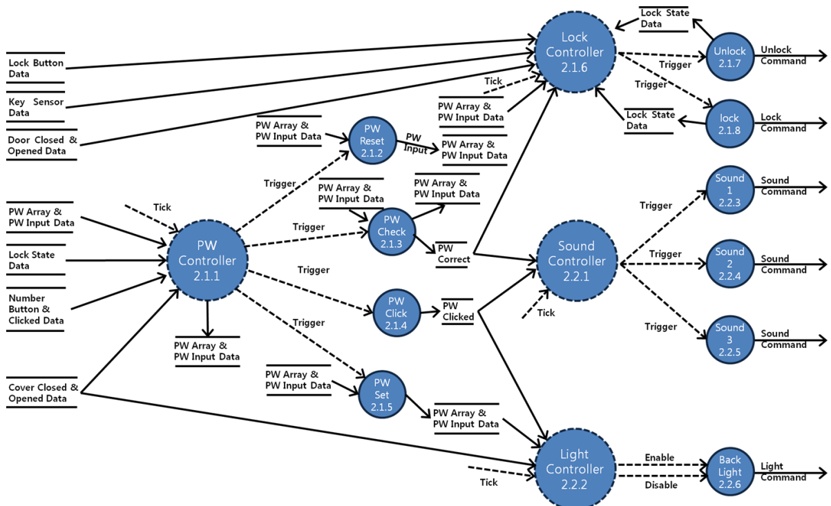
3.2.4.1.5 DFD overall for Level 3
