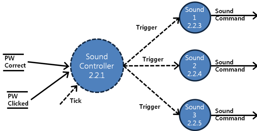
3.2.4.1.4 DFD enlarge for Light Controller & process 2.2.6
