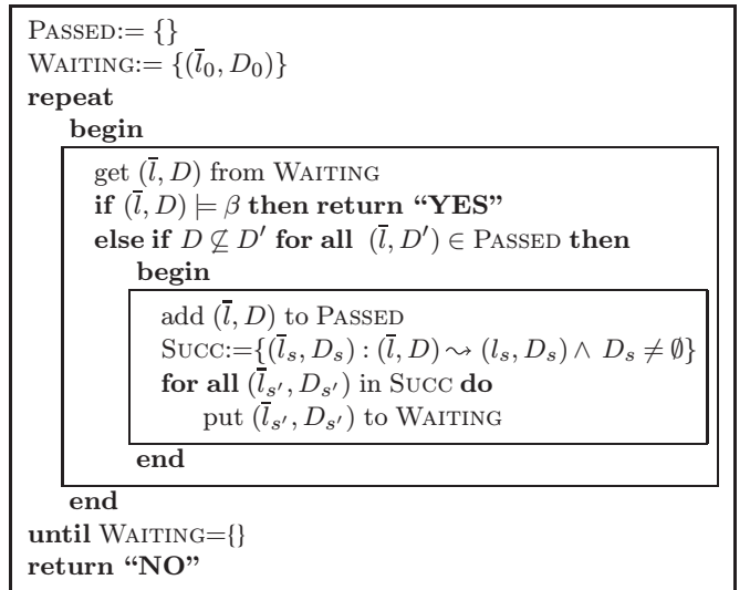
Fig. 6. An algorithm for symbolic reachability analysis
