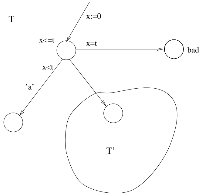
Fig. 5. Test Automata for \phi \text{ until}_t a
