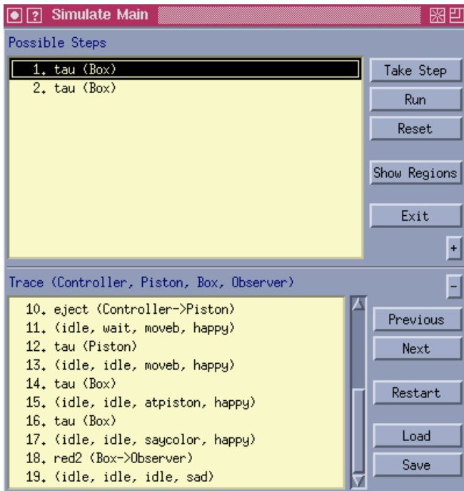
Fig. 15. The Main window
